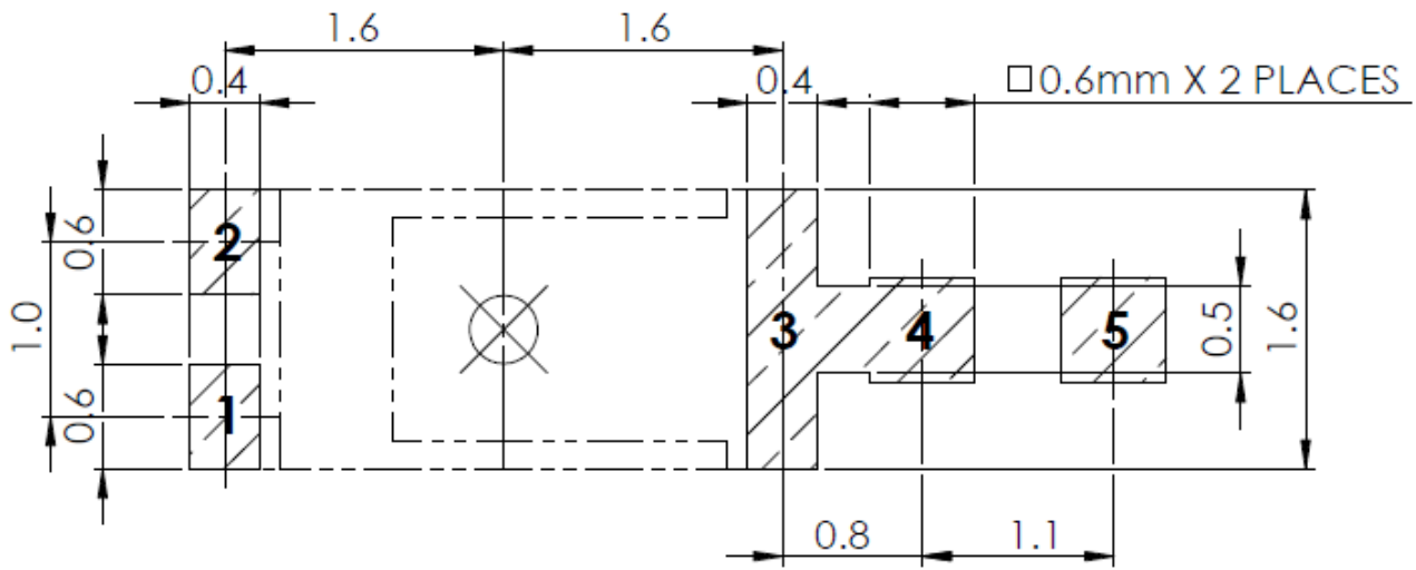
PCB FOOTPRINT
